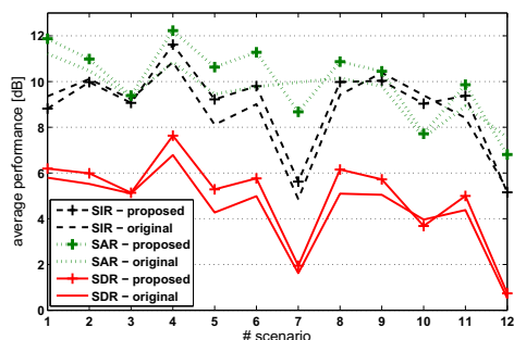
Figure 1: Detailed performance of compared approaches in all scenarios of SiSEC 2010 data.
